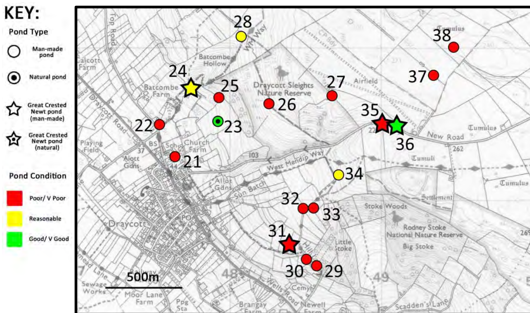
Figure 6: Cluster 3.
