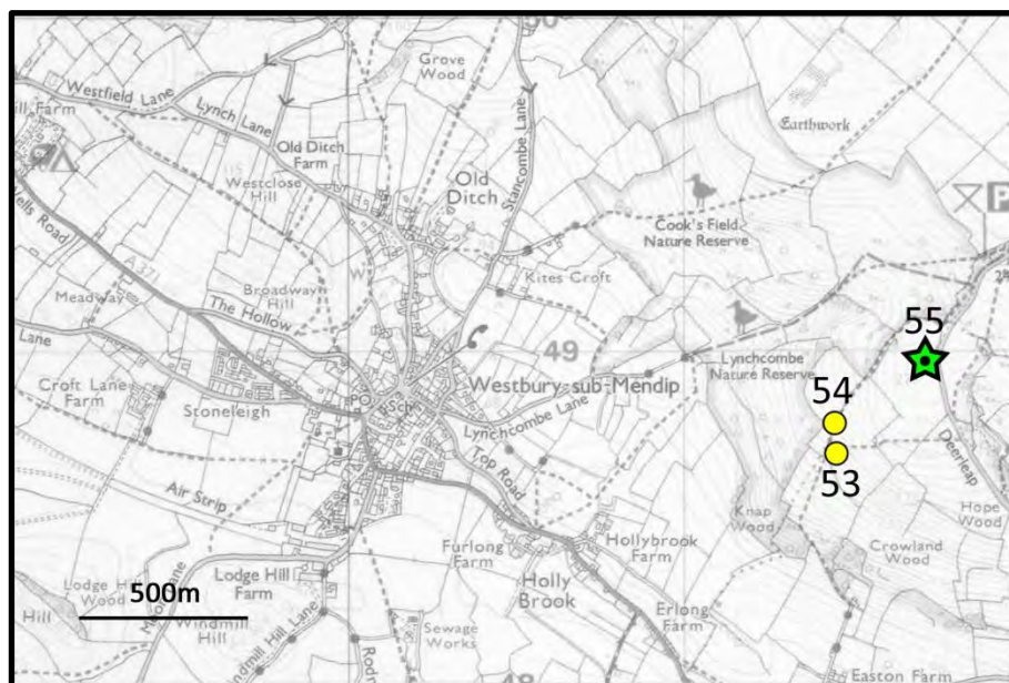
Figure 9: Cluster 6.
