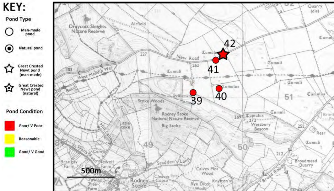
Figure 7: Cluster 4.
