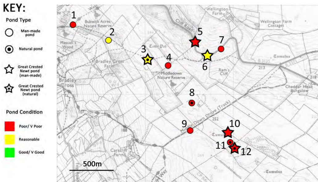
Figure 4: Cluster 1.
